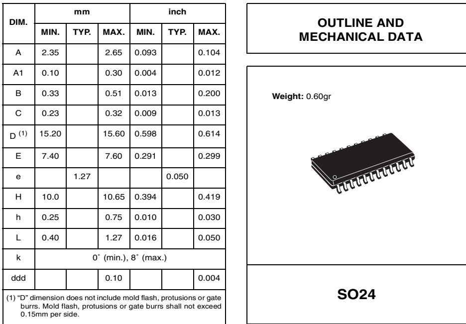
Figure 17. SO24 Mechanical Data & Package Dimensions
